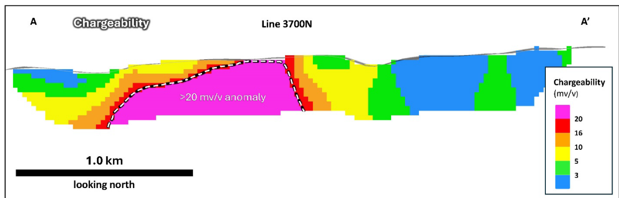
Figure 3. Section through the M5 chargeability 3D voxel model showing the strong-chargeability anomaly which has never been drill tested. Section line 3700N A to A' shown in Figure 2.
