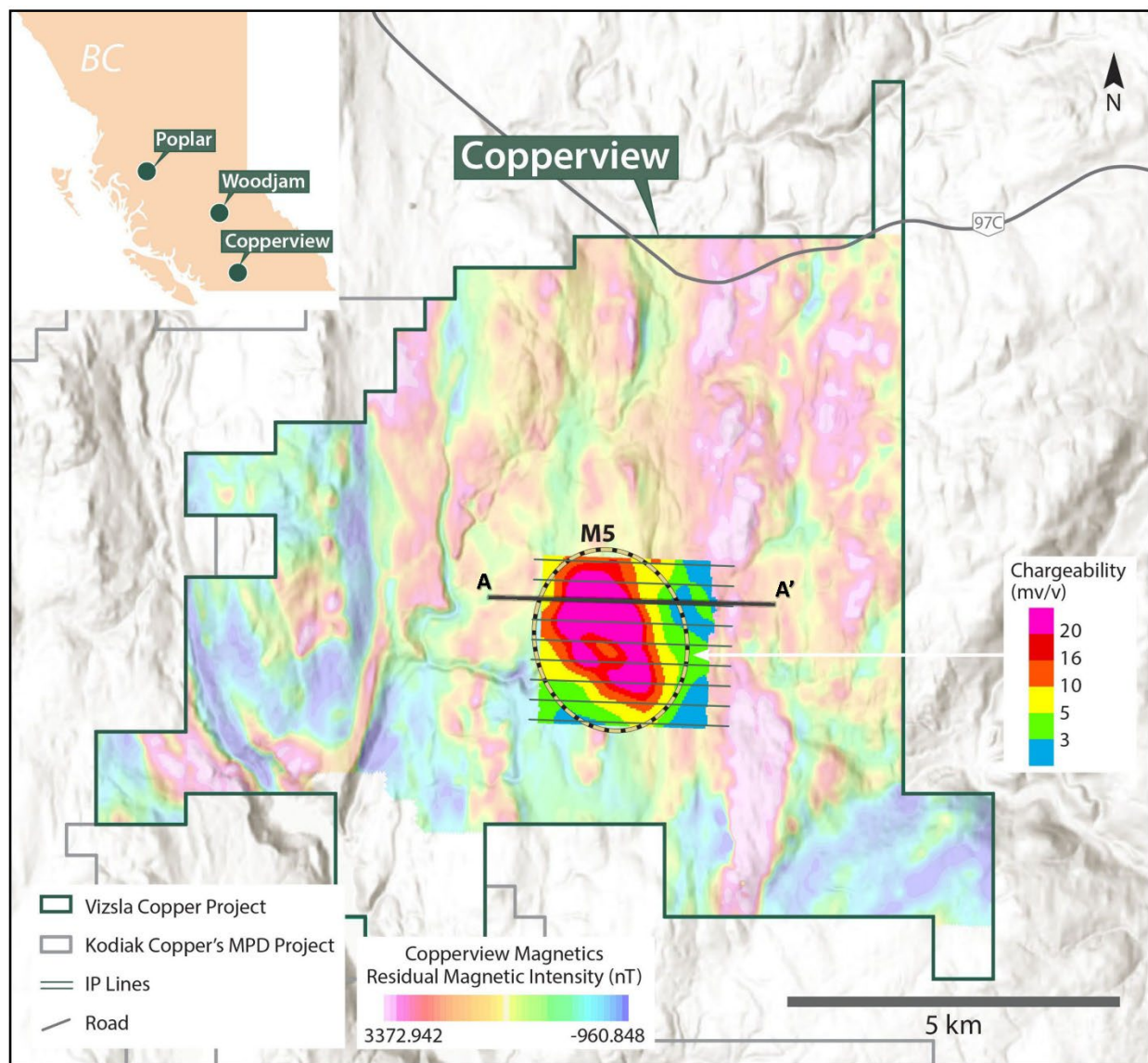
Figure 2. Project scale high-resolution magnetic data showing the location of the IP survey and the strong chargeability anomaly across the M5 target (250m depth slice).
